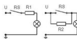
Fig. 5 Lamp loads with parallel or serial resistor to switch.
